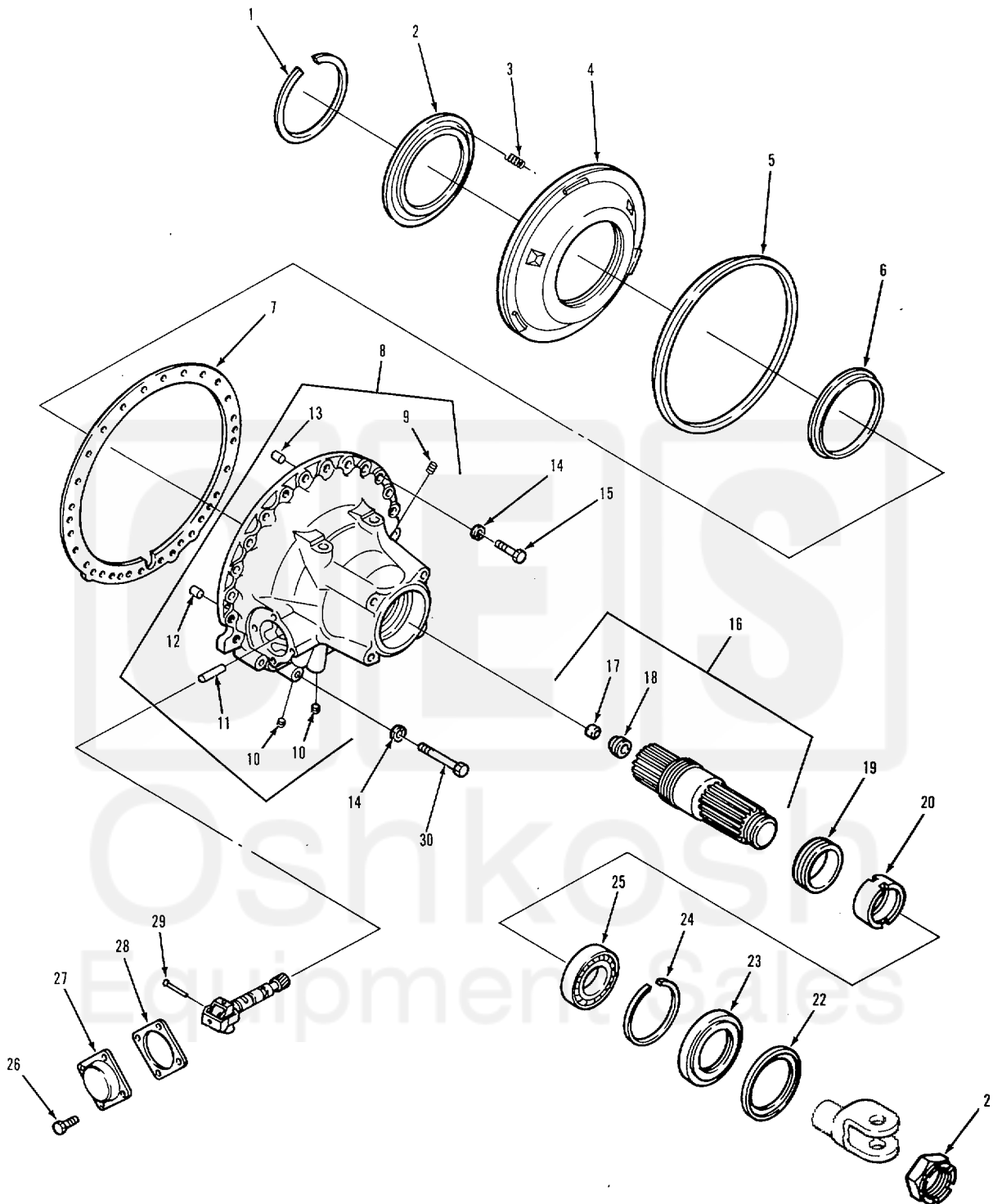
FIGURE 66. REAR HOUSING.
